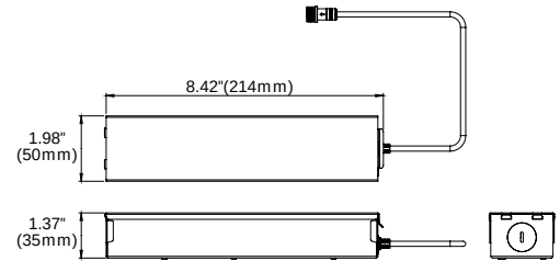
(RECESSED APPLICATION)
