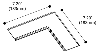
36442-013 Connecting Bracket
