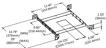
TRIM & TRIMLESS AT/IC Box: 44367-015 IC Box: 44299-019
